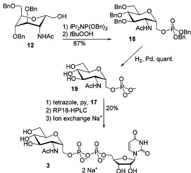
Scheme 4. Synthesis of the known C-glycoside 3
