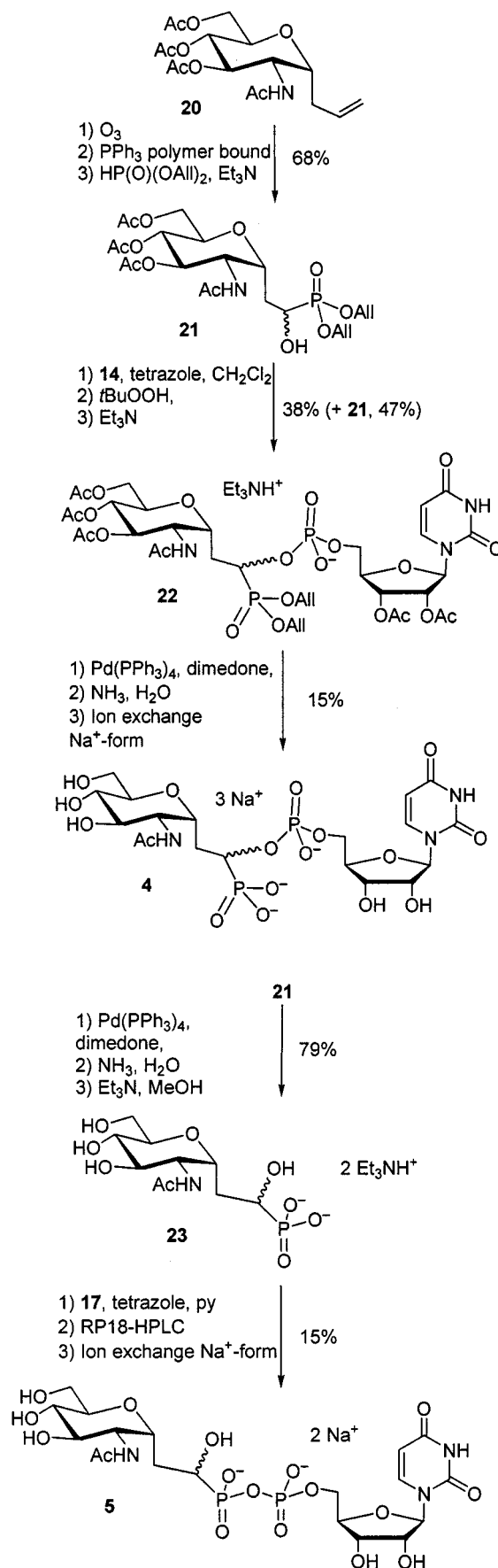
Scheme 5. Synthesis of inhibitors 4 and 5
