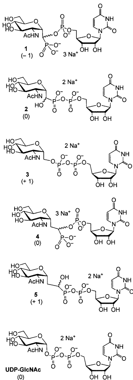
Scheme 1. Formal distance between the uridine and the sugar moiety in the synthesized inhibitors 1–5 compared with the substrate UDP-GlcNAc
