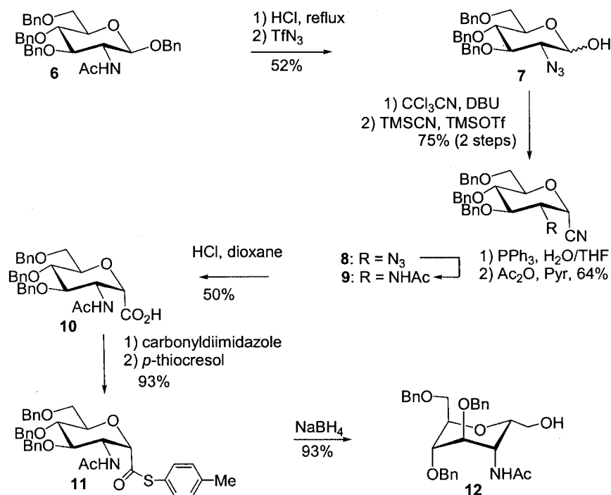
Scheme 2. Synthesis of heptitol 12
