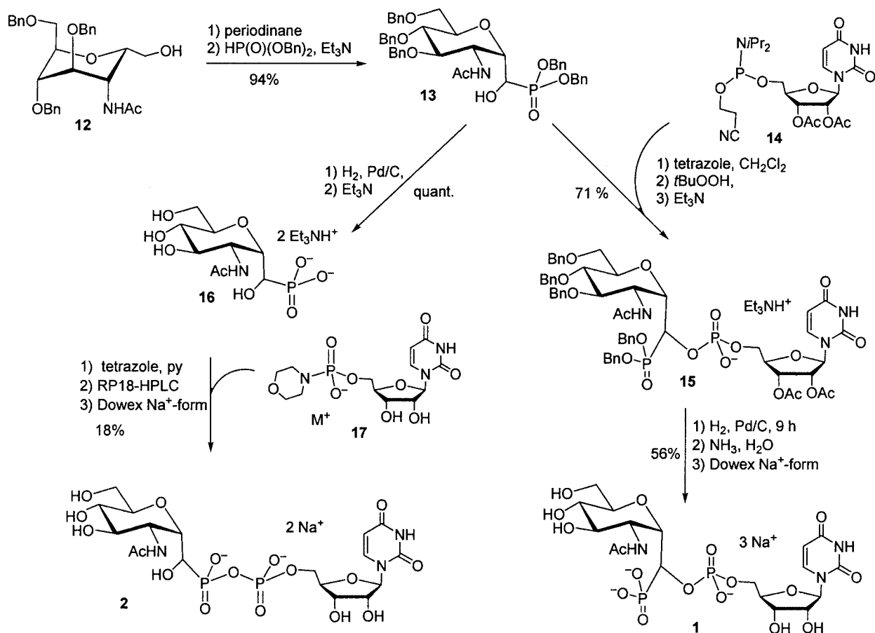
Scheme 3. Synthesis of the target molecules 1 and 2
